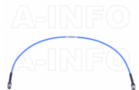
2.4M-2.4M-B020-500 Flexible Cable Assembly 500mm DC-50GHz 2.4mm Male to 2.4mm Male
